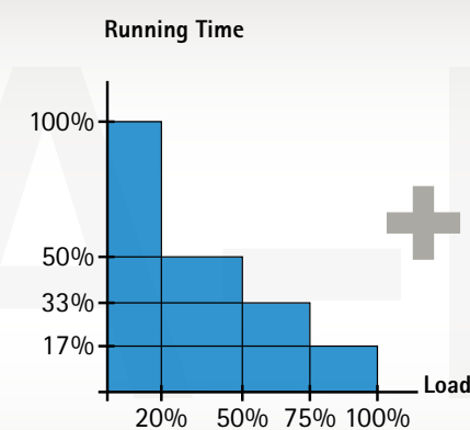
Average capacity utilisation of an industrial crane*
